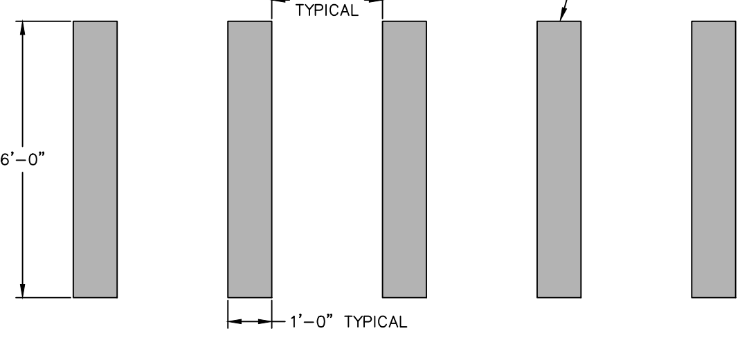
PAINTED CROSSWALK DETAIL NOT TO SCALE
