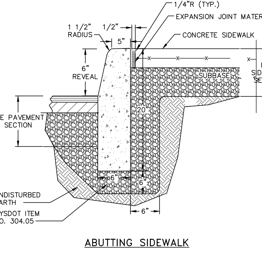
ABUTTING SIDEWALK
