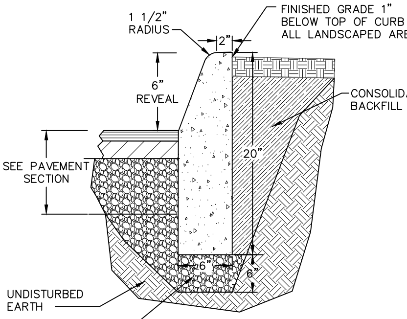
MOUNTABLE CURB ABUTTING GRASS OR LANDSCAPE NOT TO SCALE
