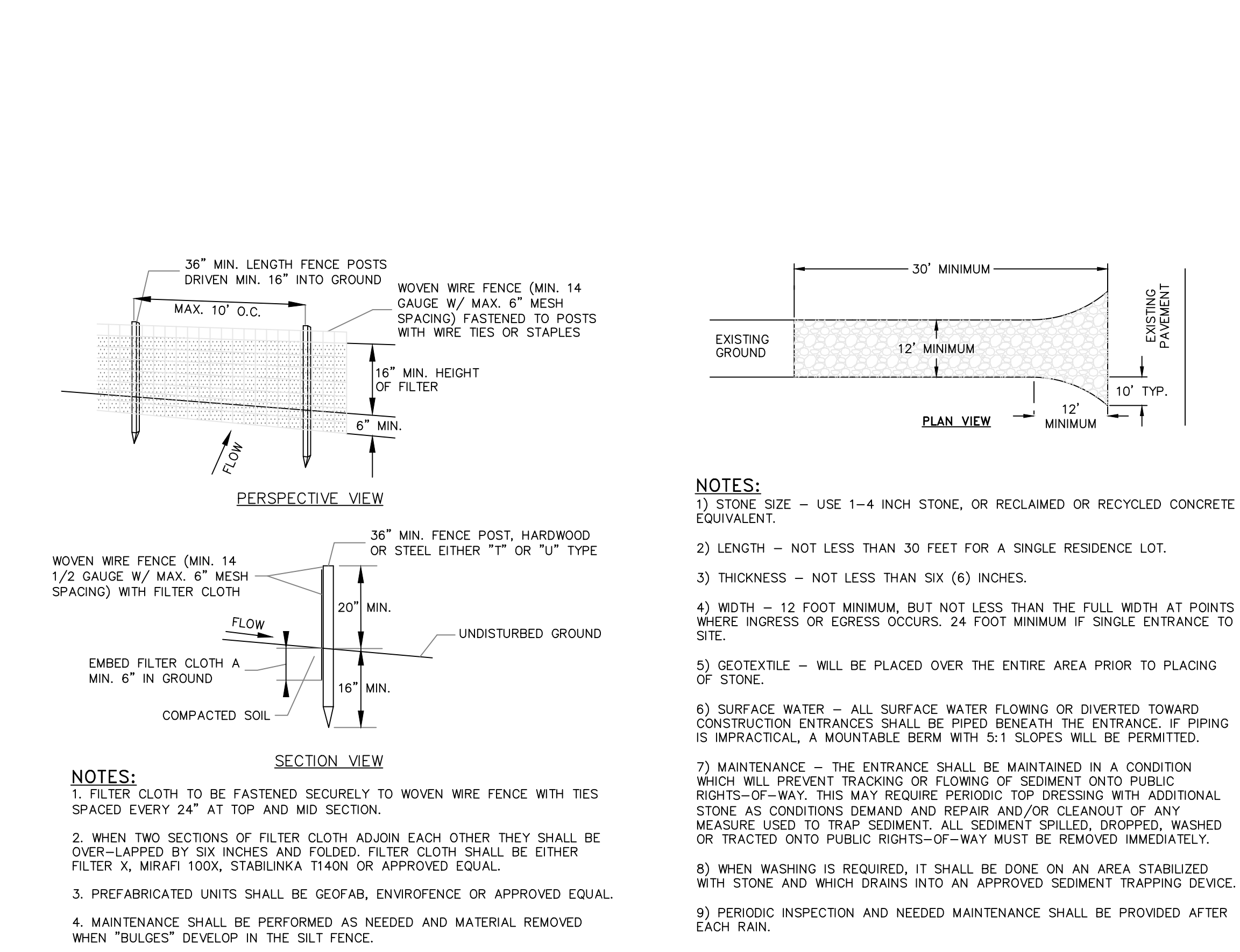
SILT FENCE DETAIL NOT TO SCALE
