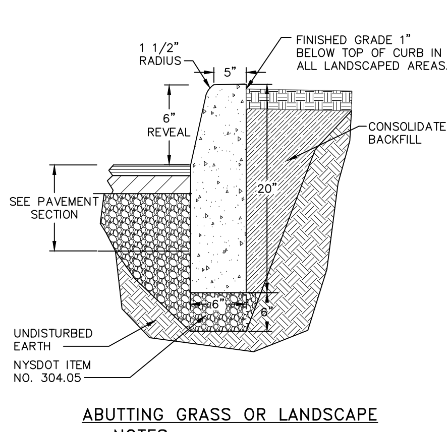
ABUTTING GRASS OR LANDSCAPE
