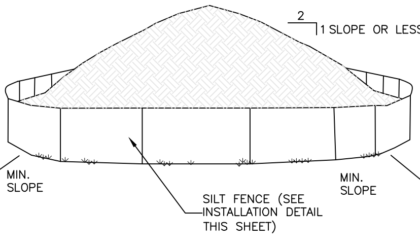
TEMPORARY SOIL STOCKPILE DETAIL NOT TO SCALE
