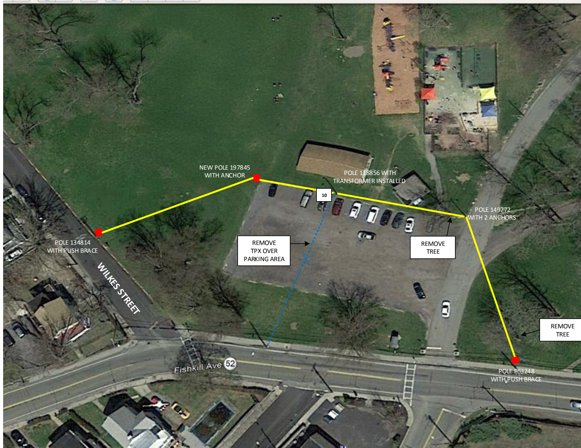
J772683- ROUTE OF NEW CENTRAL HUDSON CONDUCTOR THRU BEACON PARK - CITY OF BEACON
