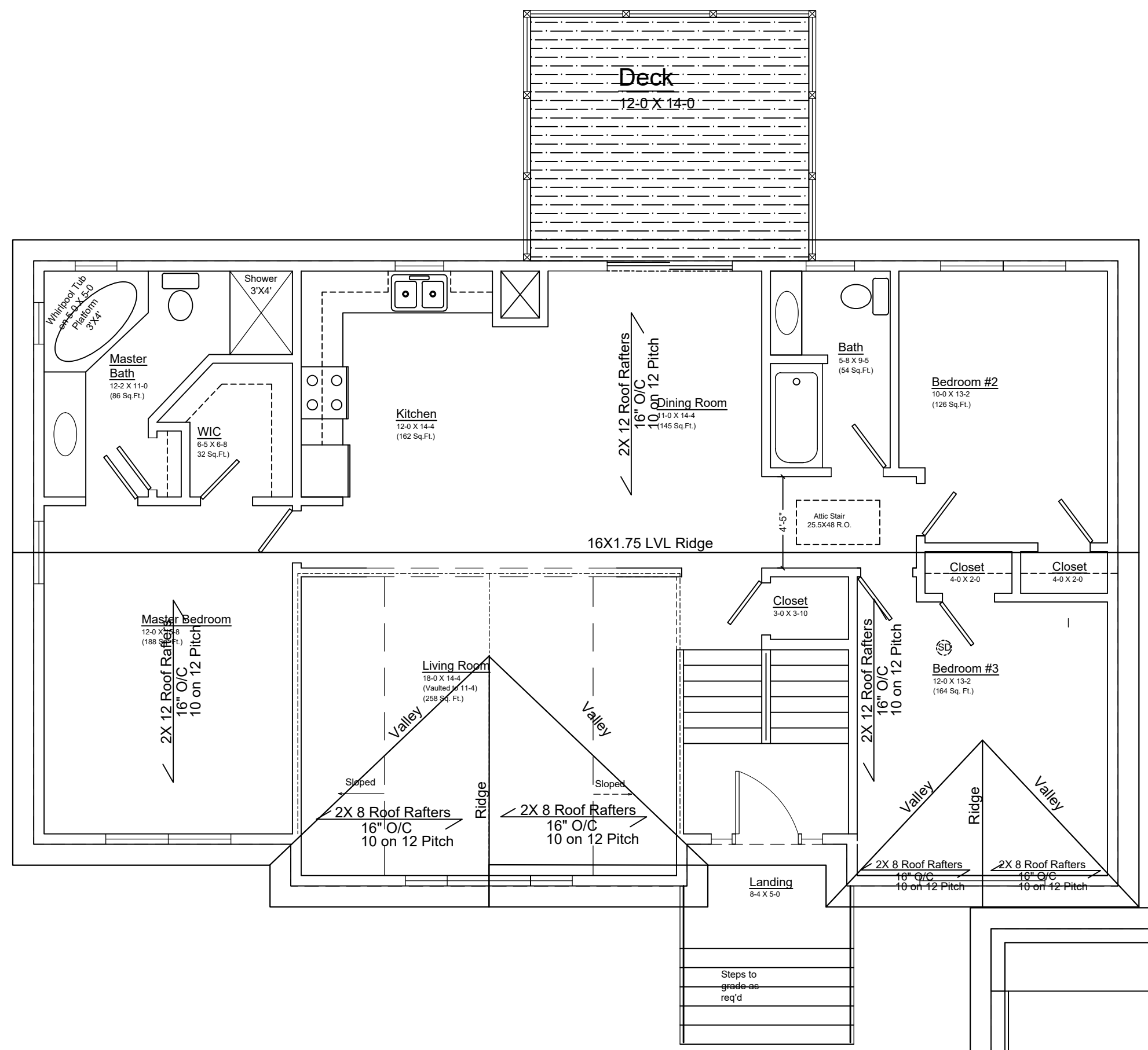
1 Upper Level Floor Plan SCALE: 3/8" = 1'-0"
