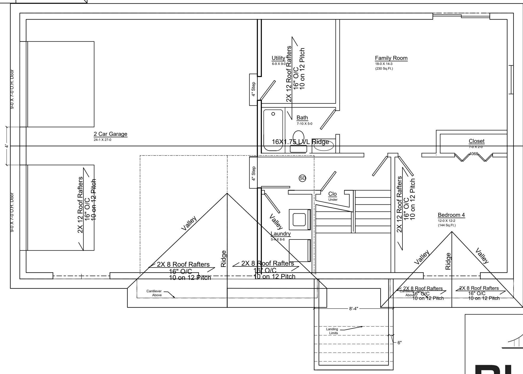
1 Lower Level Floor Plan SCALE: 3/8" = 1'-0"
