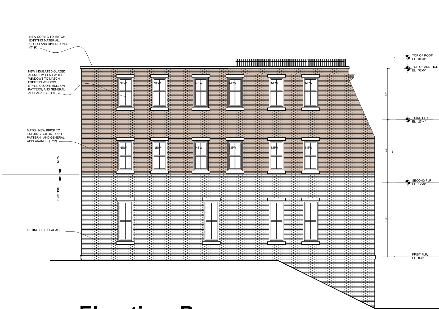
Elevation: Rear
