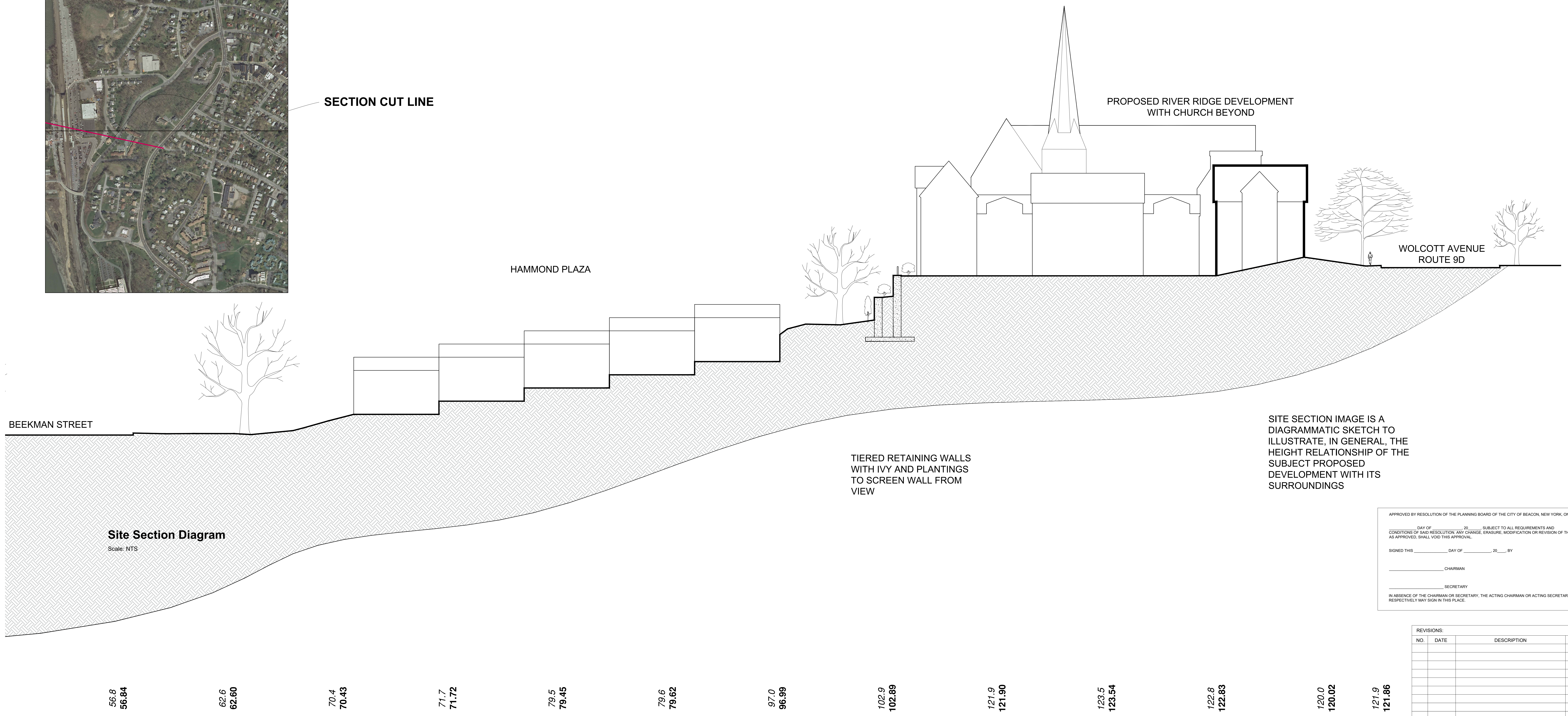
Site Section Diagram
