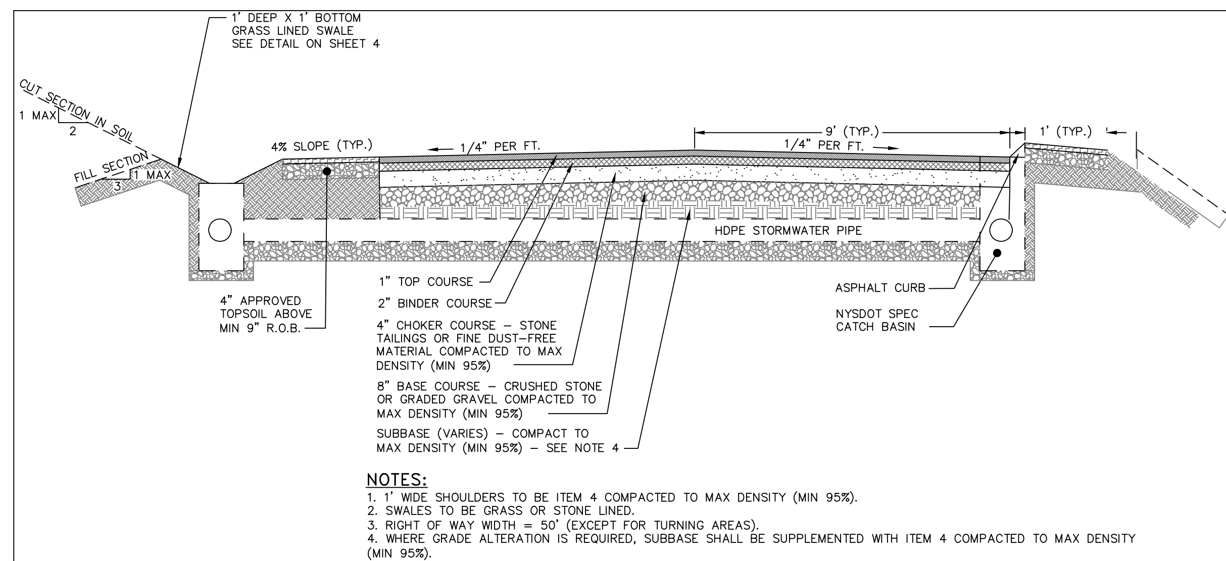
CITY OF BEACON PRIVATE ROAD SECTION SCALE: NOT TO SCALE
