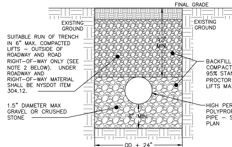
STORM LINE TRENCH DETAIL NOT TO SCALE
