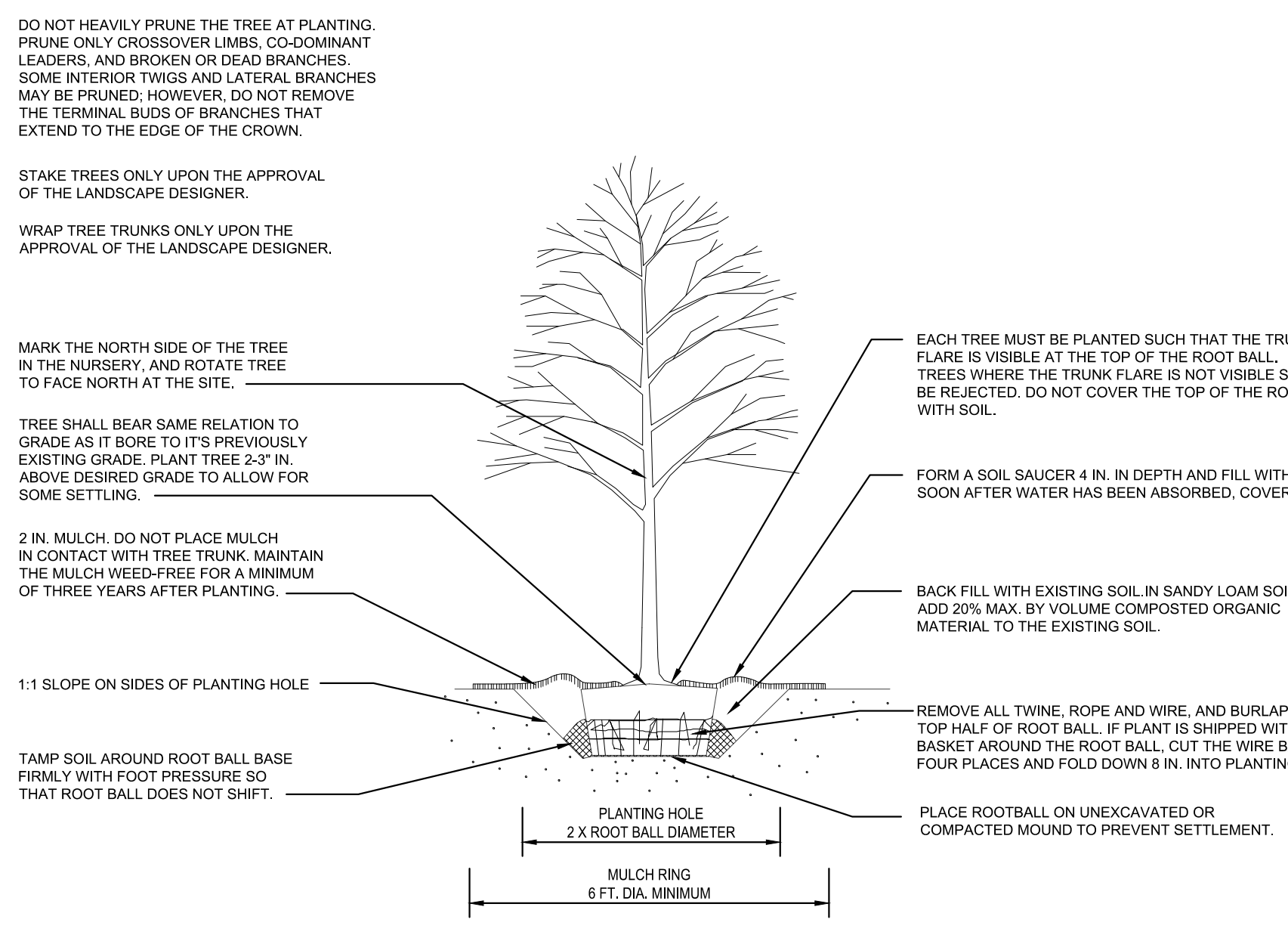
TREE PLANTING DETAIL NOTE: THIS DETAIL ASSUMES THAT THE PLANTING SPACE IS LARGER THAN 8 FT. SQUARE, OPEN TO THE SKY, AND NOT COVERED BY ANY PAVING OR GRATING.
