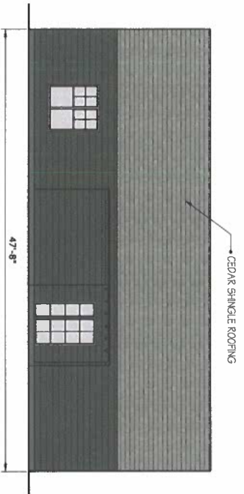
FRONT ELEVATION
