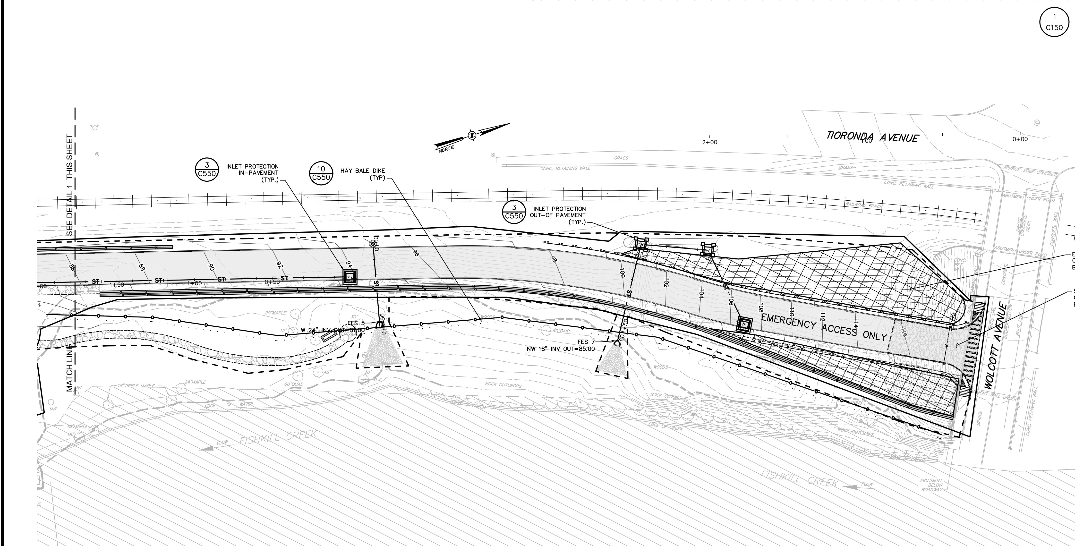
2 EROSION AND SEDIMENT CONTROL PLAN SCALE: 1"=30'
