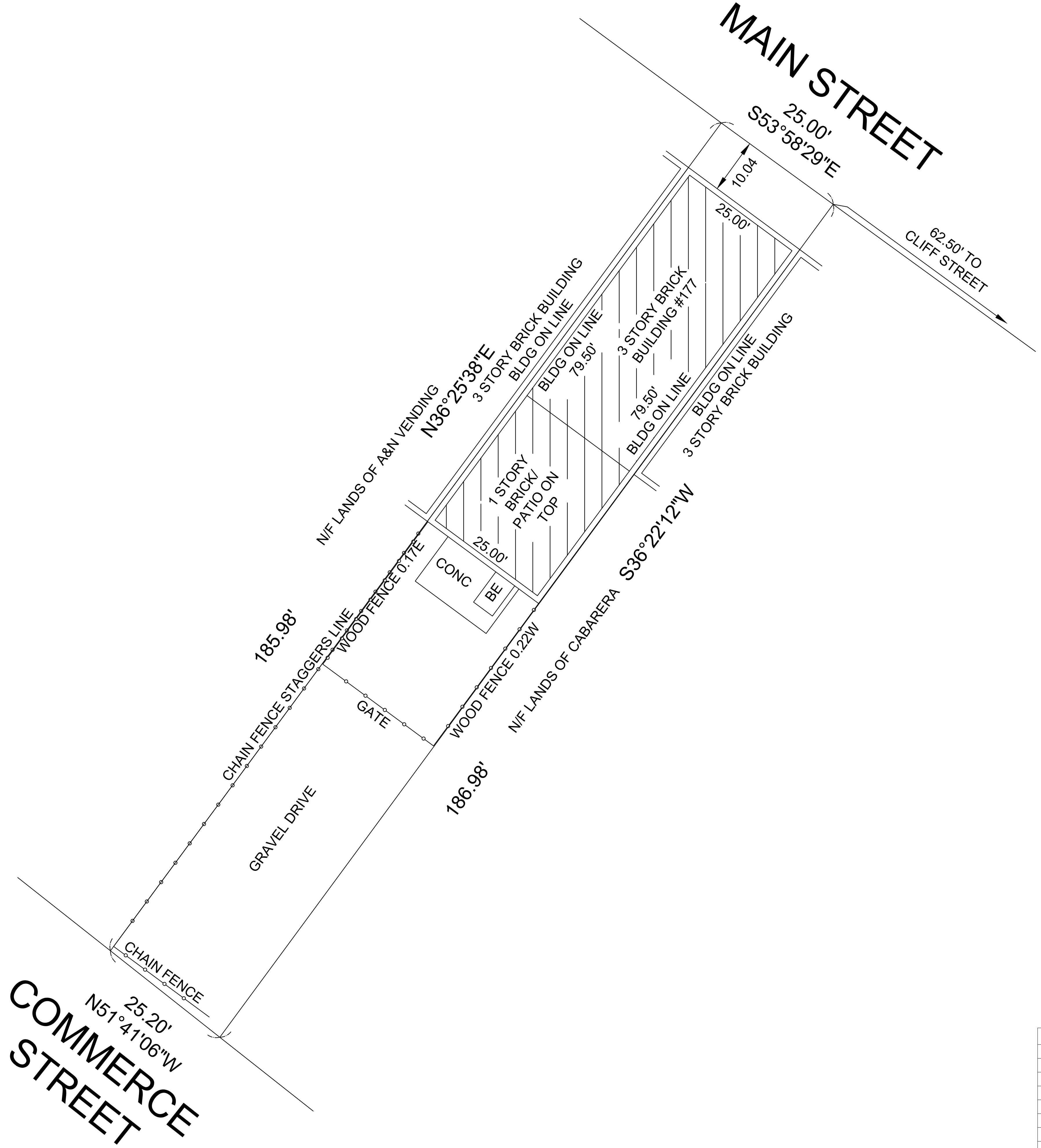
Existing Conditions Plan Scale: 1" = 10'
