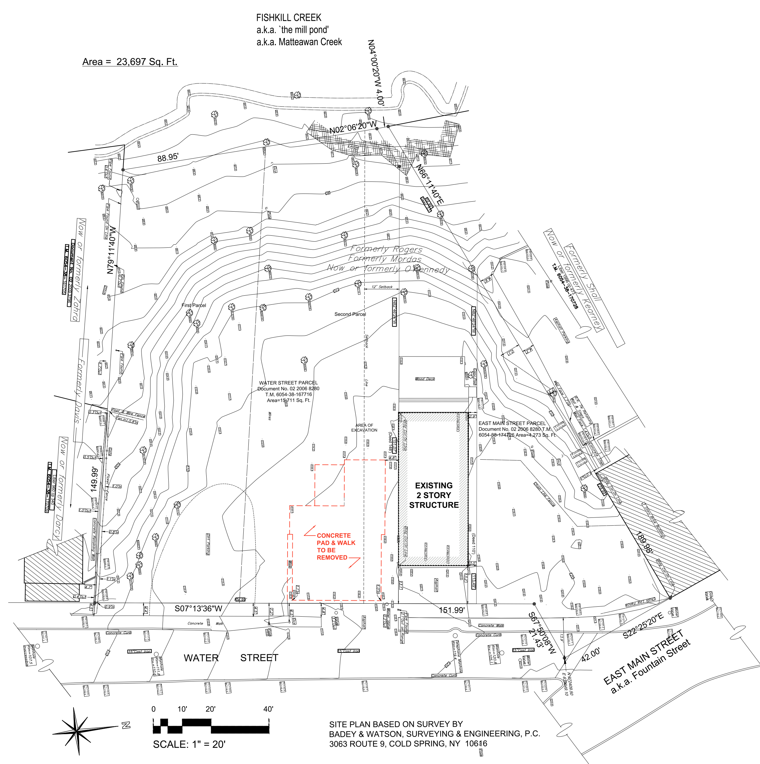
Site Demolition Plan Scale: 1" = 20'
