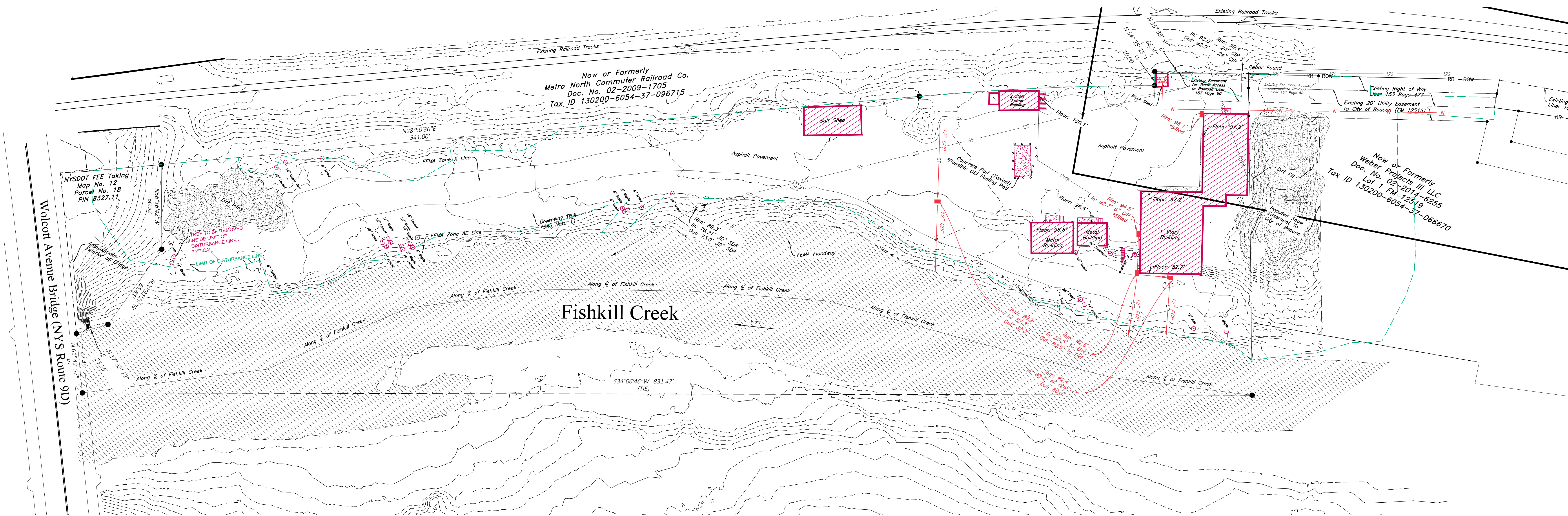
Demolition Plan
