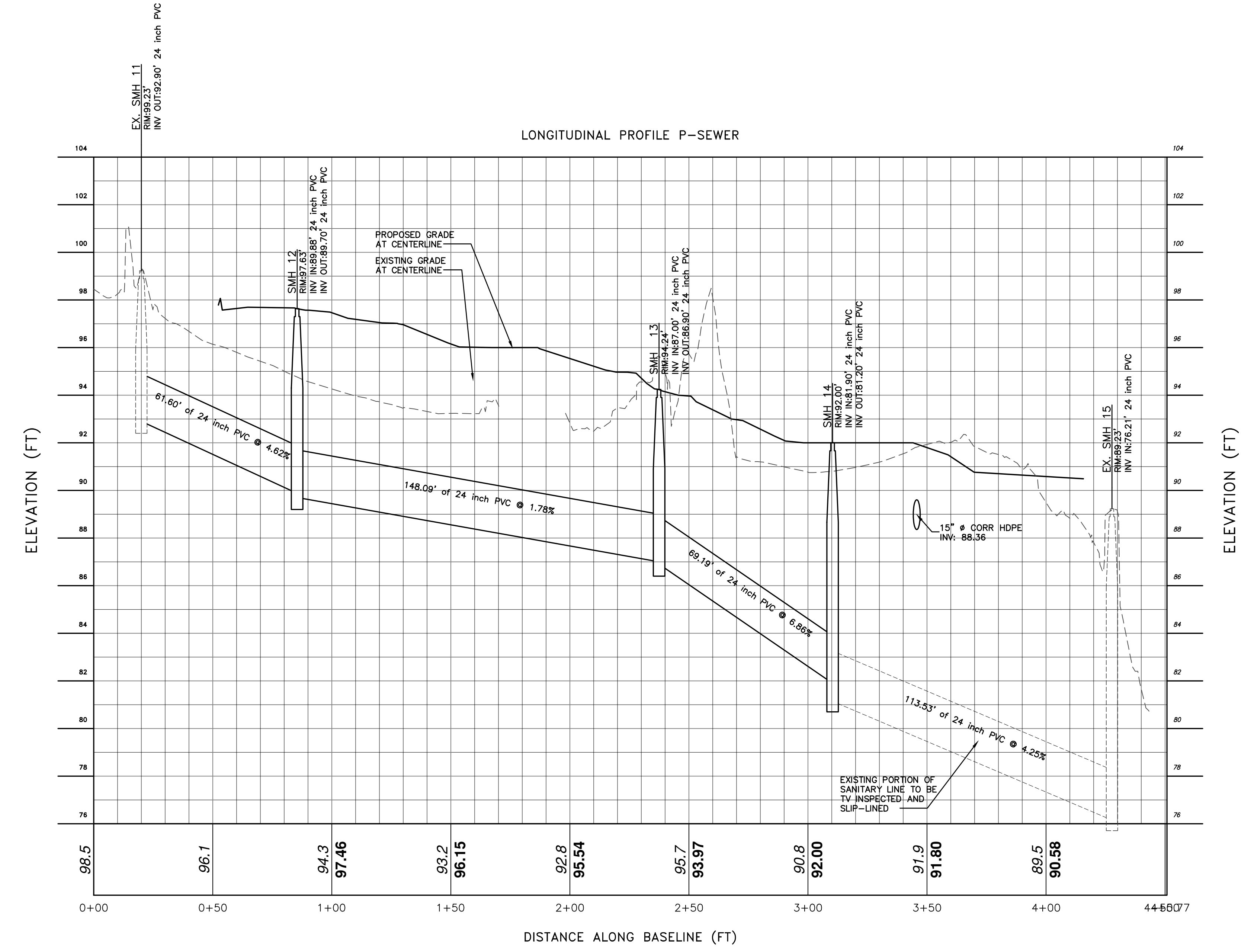
SEWER LINE PROFILE SCALE: 1" = 3'V 1" = 30'H
