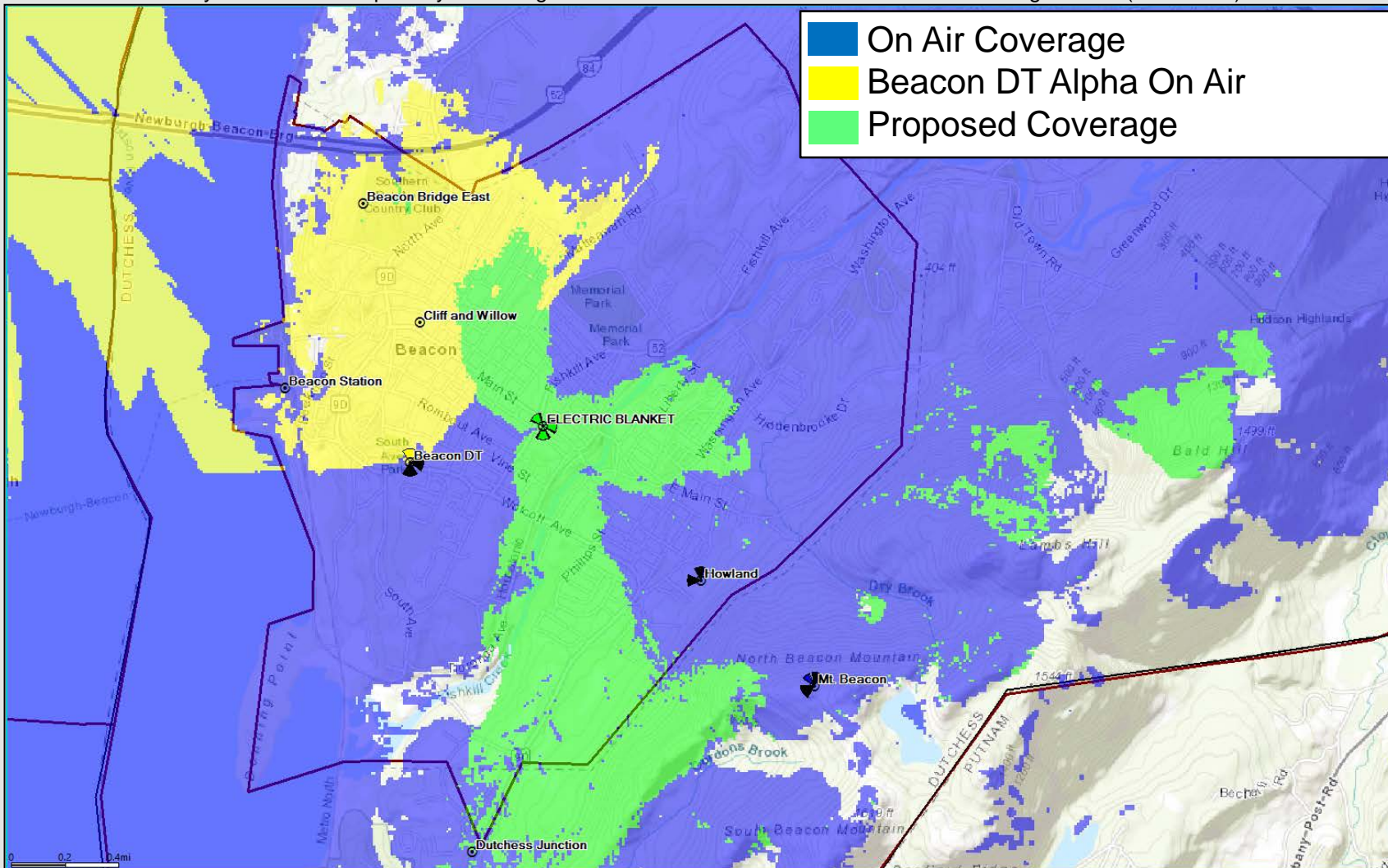
The map above removes the footprint of the existing Mt. Beacon site showing the improved benefit and coverage footprint of the proposed Electric Blanket site (green coverage).
