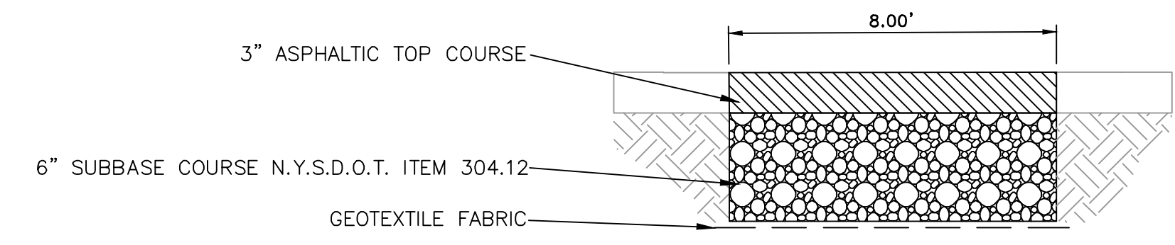
WALKWAY DETAIL NOT TO SCALE
