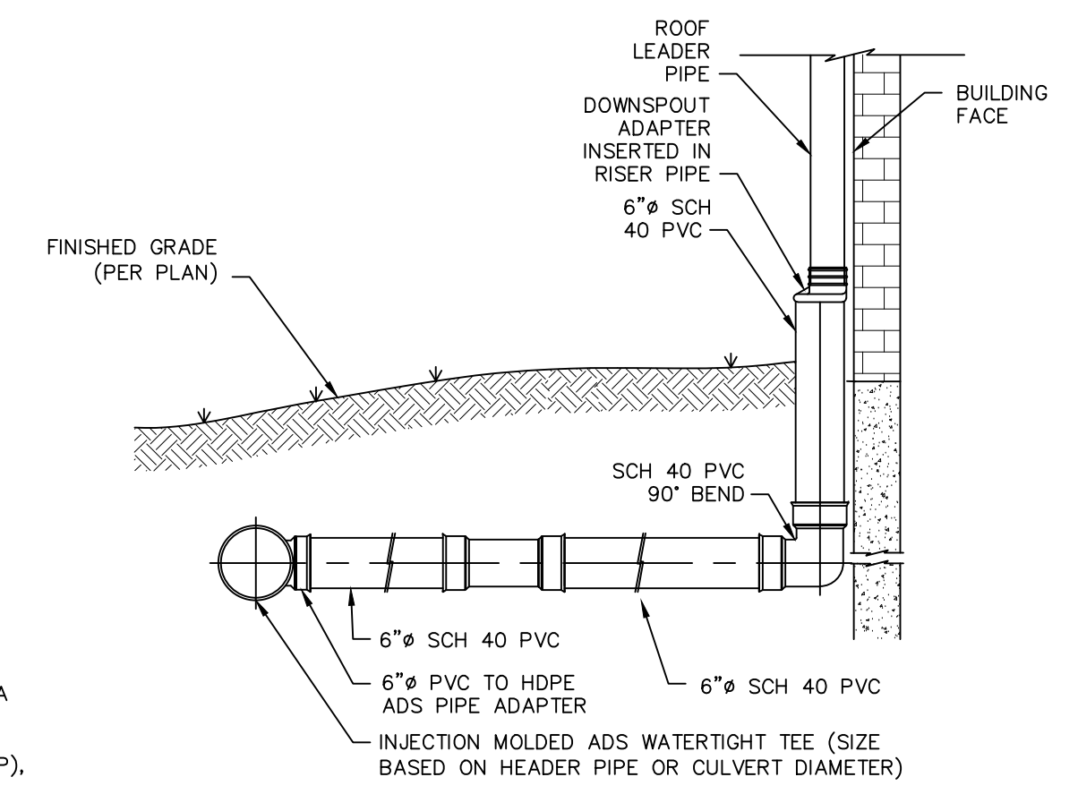
ROOF LEADER CONNECTION DETAIL NOT TO SCALE
