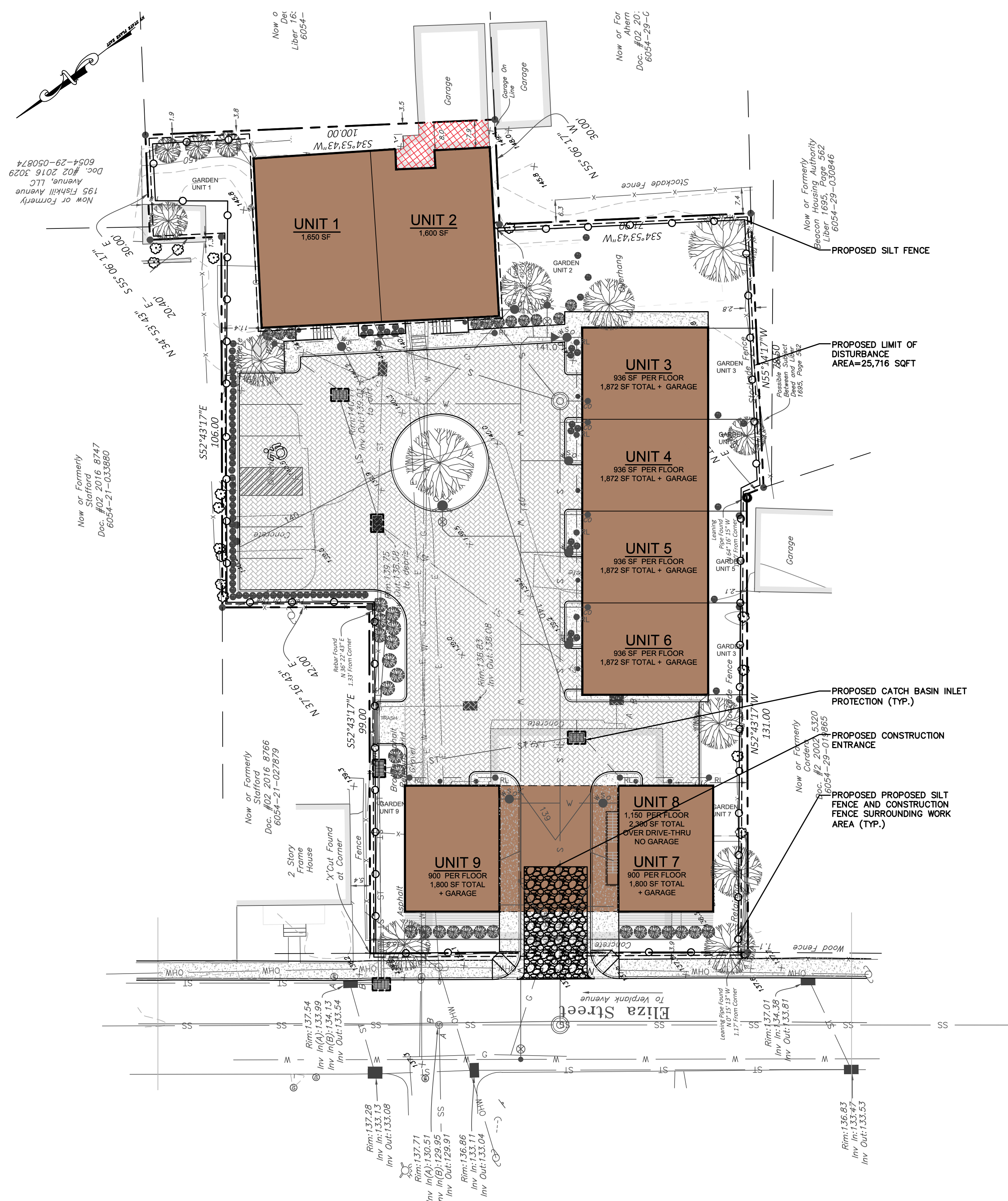
EROSION & SEDIMENT CONTROL PLAN SCALE: 1" = 20' GRAPHIC SCALE ( IN FEET ) 1 inch = 20 ft.
