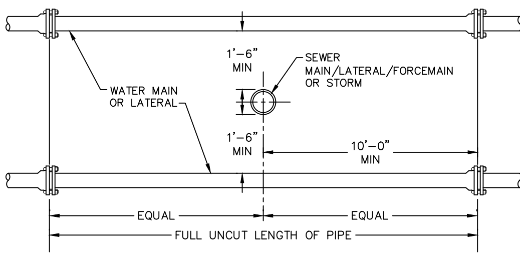
VERTICAL SEPARATION
