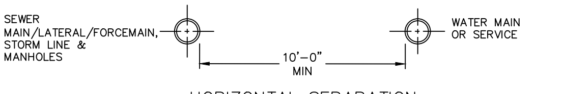
HORIZONTAL SEPARATION
