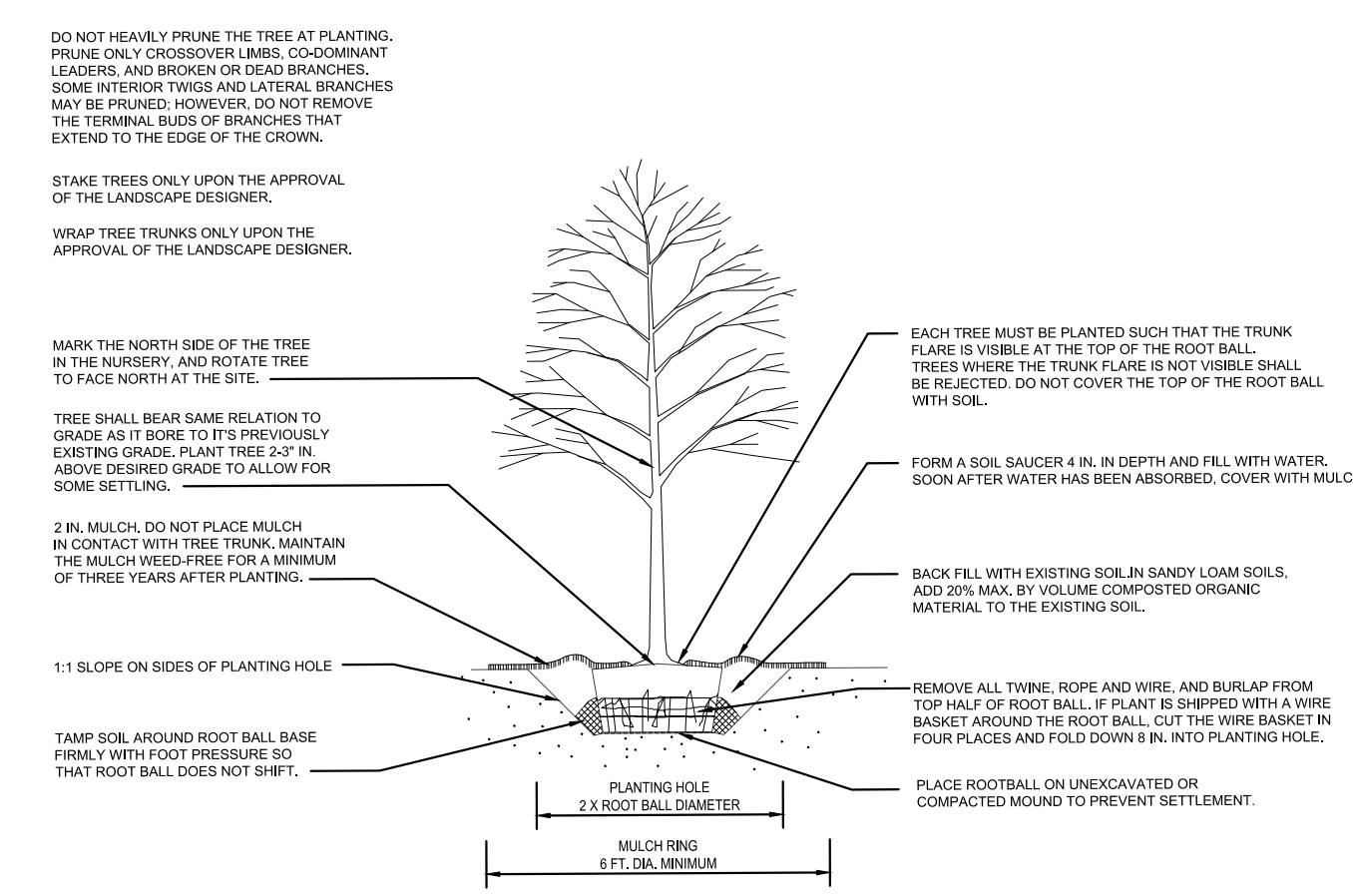
NOTE: THIS DETAIL ASSUMES THAT THE PLANTING SPACE IS LARGER THAN 6 FT. SQUARE, OPEN TO THE SKY, AND NOT COVERED BY ANY PAVING OR GRATING.
